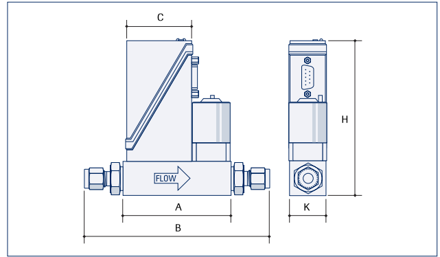
IP40 Mass Flow Controller
