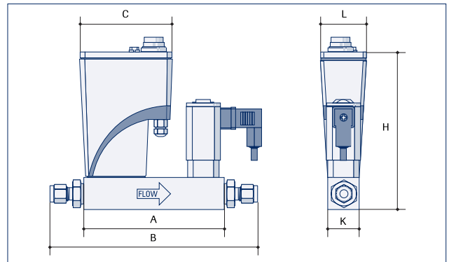
IP65 Mass Flow Controller
