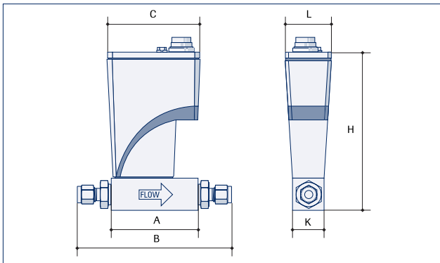
IP65 Mass Flow Meter, low/medium flow
