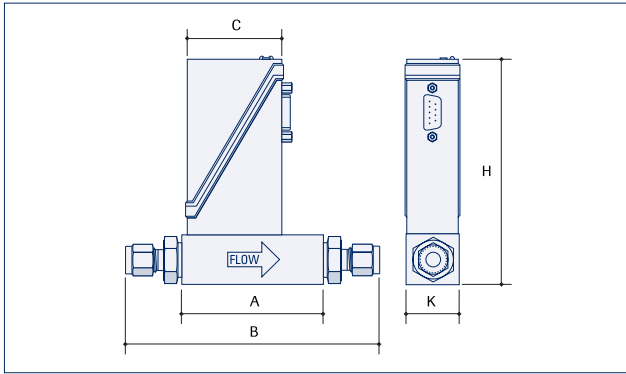
IP40 Mass Flow Meter
